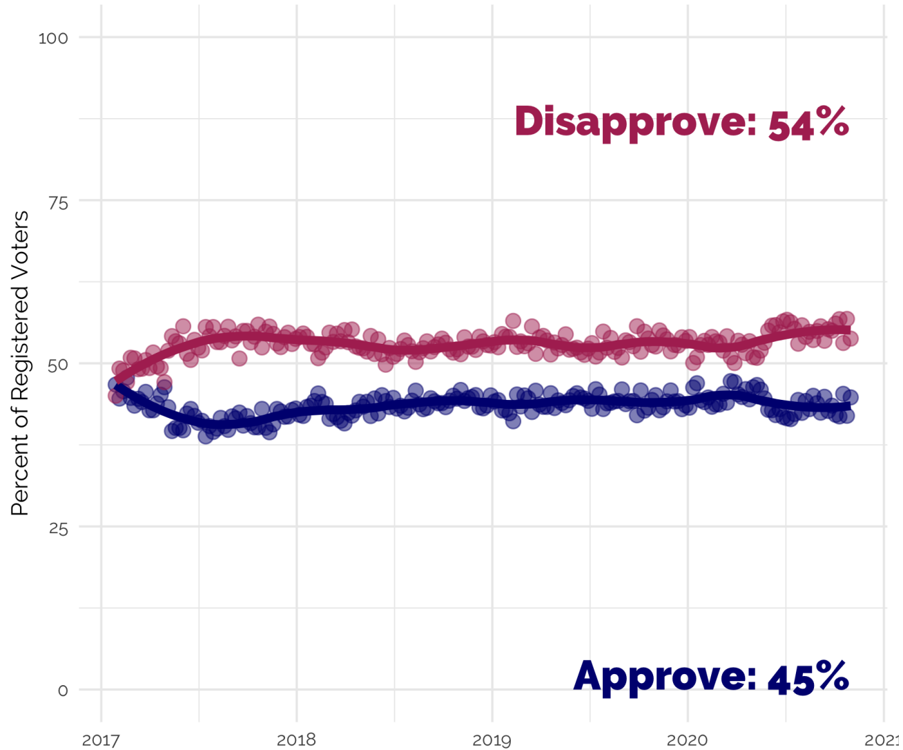
Figure 1: Trump Approval – Registered Voters
